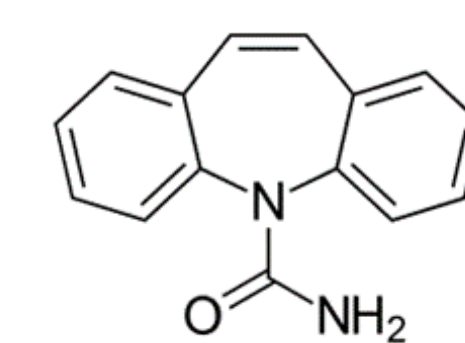
Carbamazepine
